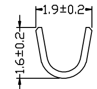
B-B SEC
